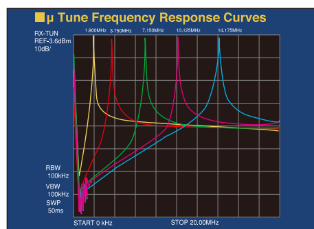
■ 10dB/Div·2MHz/Div
