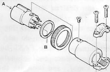
Plug assembly
