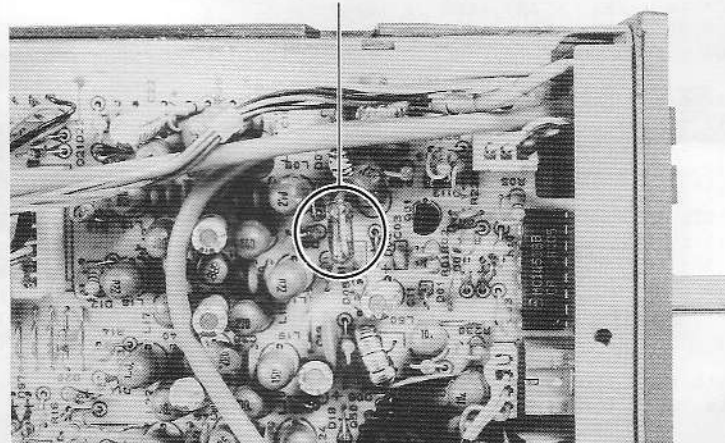
LAMP FUSE (F 1001 )
