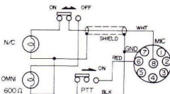
YM-36 MICROPHONE CONNECTIONS
